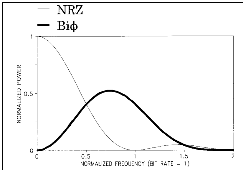
Figure A-2. Spectral Densities of Random NRZ and Bi-phase Codes
