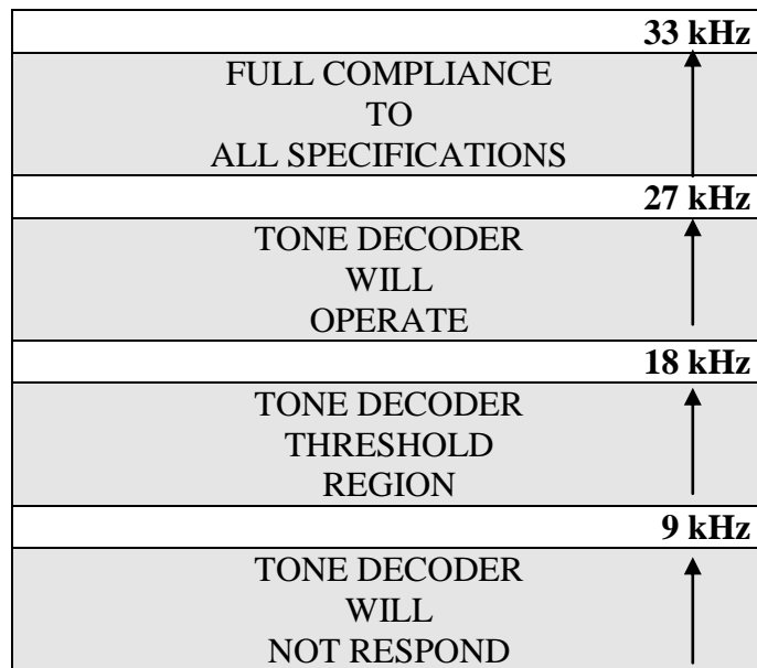
Figure 2-3. Decoder deviation.
